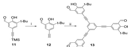
Scheme 3. Reagents and conditions: (i) KF, MeOH, rt, 1 h, 75%; (ii) 1,3,5-triiodobenzene, Pd(PPh 3 ) 2 Cl 2 , CuI, t Pr 3 NEt, THF, reflux, 12 h, 58%.
