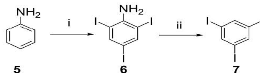
Scheme 1. Reagents and conditions: (i) HCl, H 2 O, KICl 2 , rt, 87%; (ii) H 2 SO 4 , CH 3 COOH, NaNO 2 , Cu 2 O, EtOH, reflux, 4 h, 84%.
