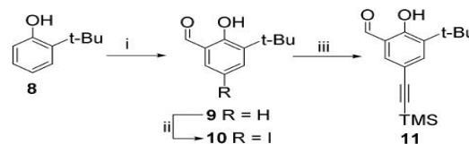
Scheme 2. Reagents and conditions: (i) SnCl 4 , leutidine, HCHO, toluene, 100 °C, 10 h, 85%; (ii) ICl, CH 3 COOH, 120 °C, 5 h, 97%; (iii) trimethylsilylacetylene, Pd(PPh 3 ) 2 Cl 2 , CuI, t Pr 3 NEt, THF, reflux, 4 h, 98%.
